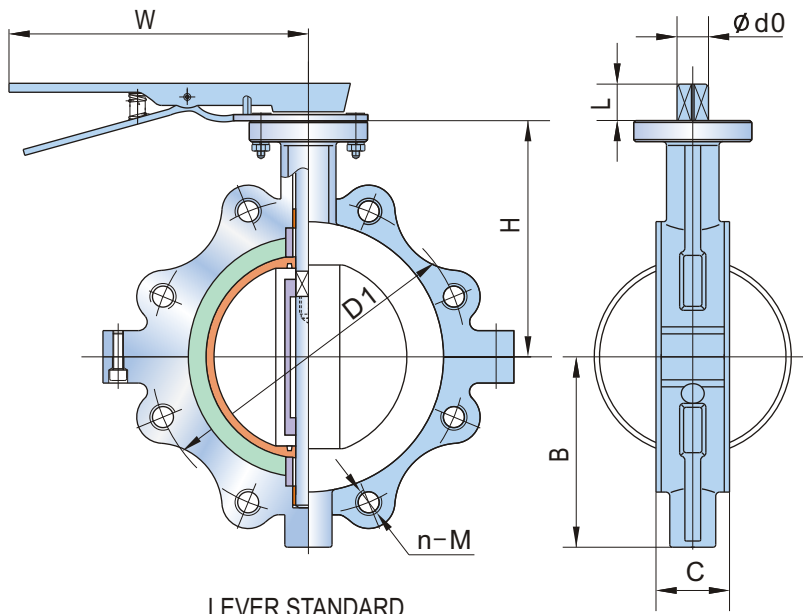
LEVER STANDARD FOR 1-1/2"-4"
