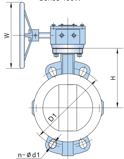
GEAR STANDARD FOR 5" & LARGER
